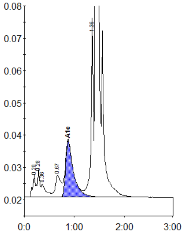
Peak table - ID: 10583449
